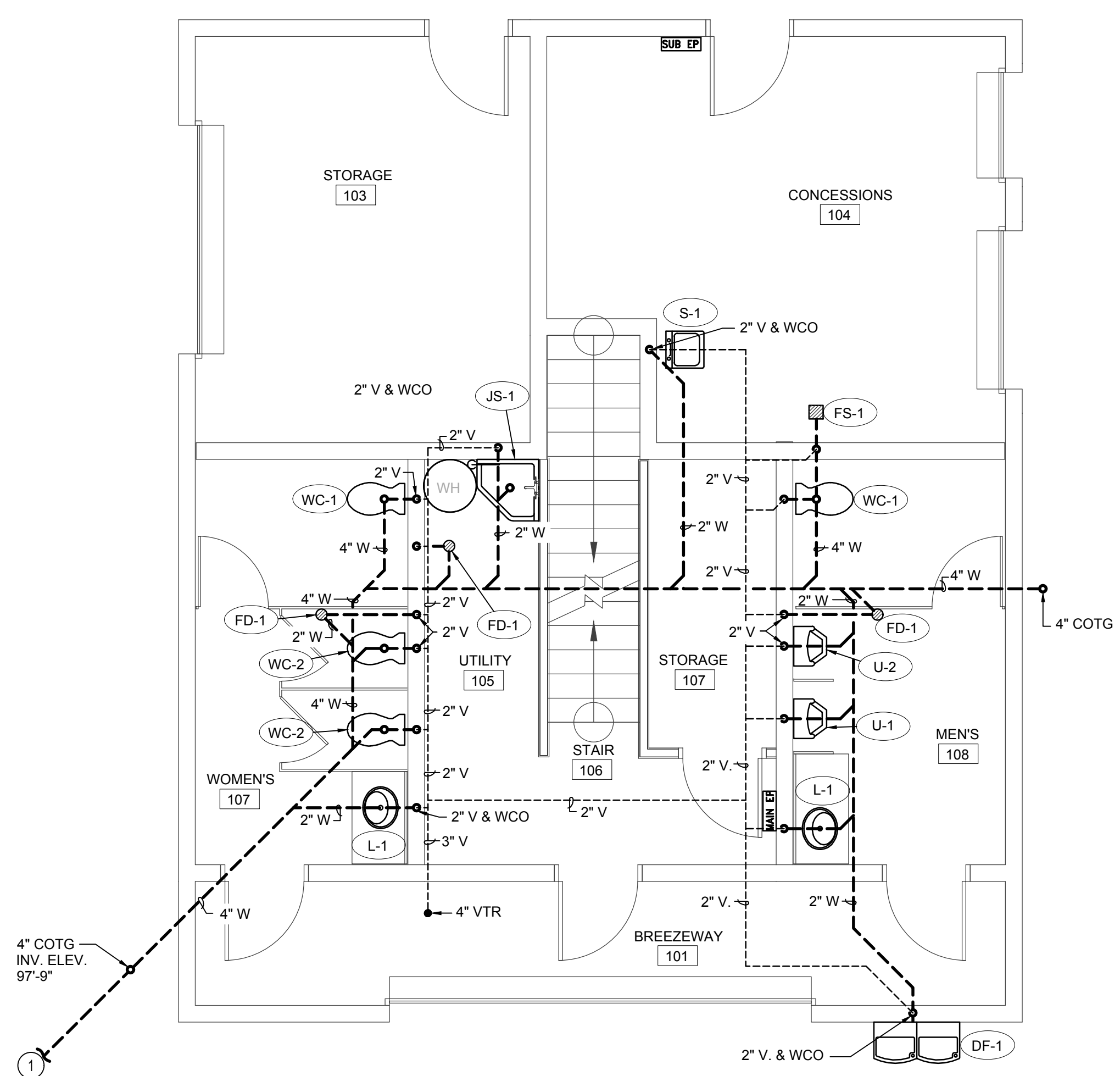
WASTE & VENT PLUMBING PLAN SCALE: 1/4" = 1'-0"
