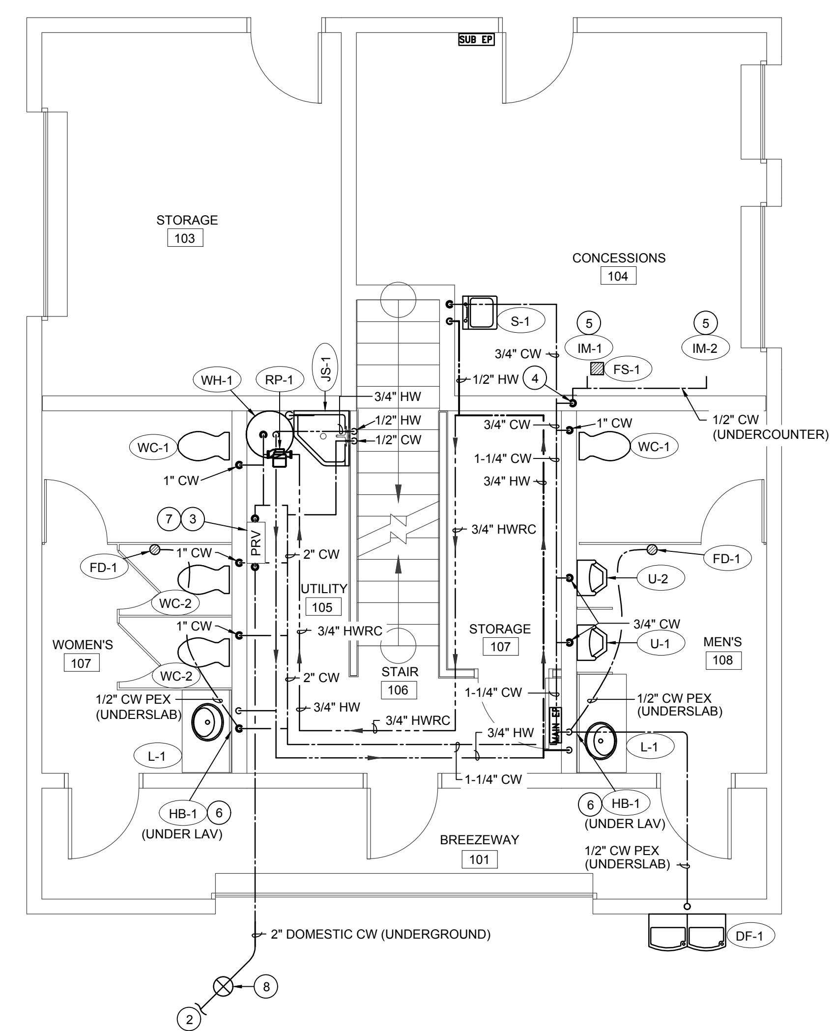
WATER PLUMBING PLAN SCALE: 1/4" = 1'-0"
